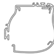
Type B 73 x 72 mm
